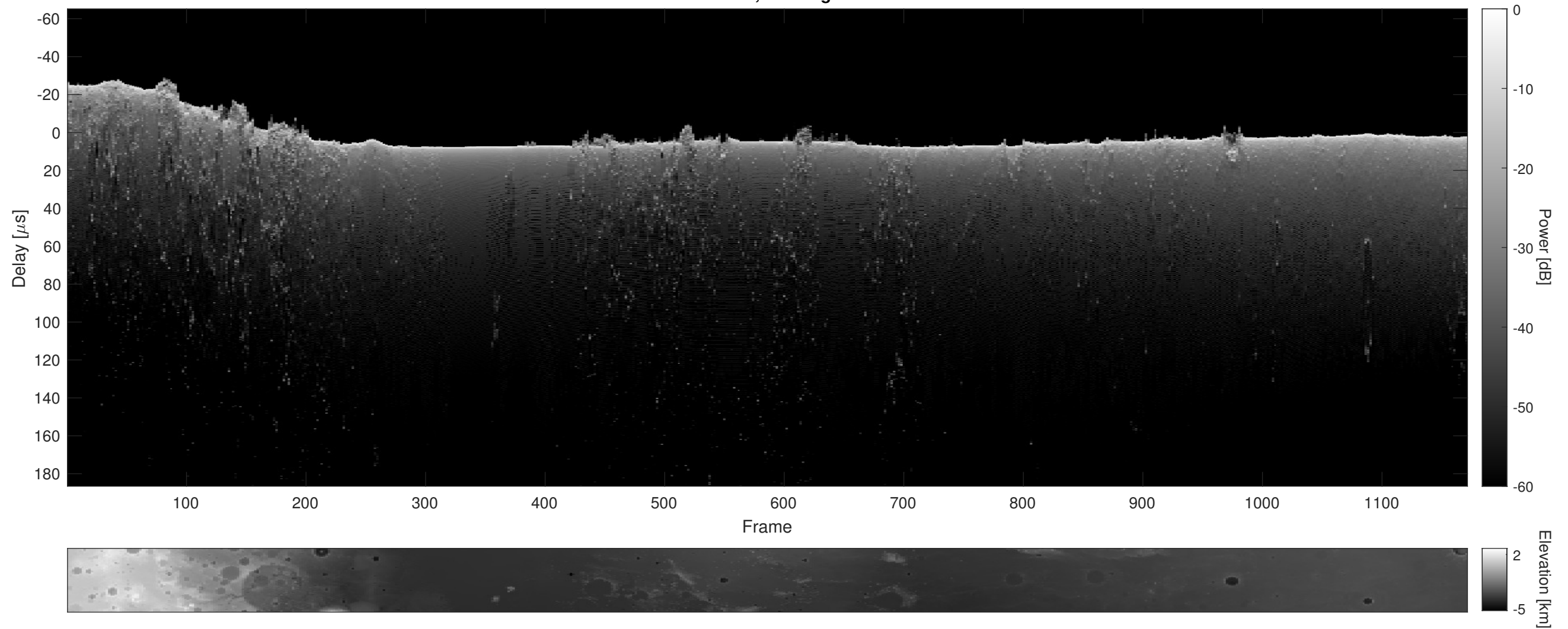
Orbit 6012, Cluttergram
