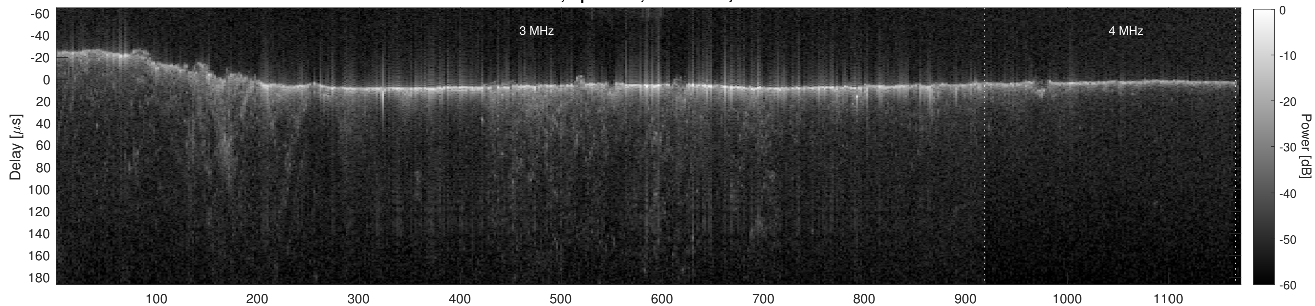
Orbit 6012, Cluttergram
