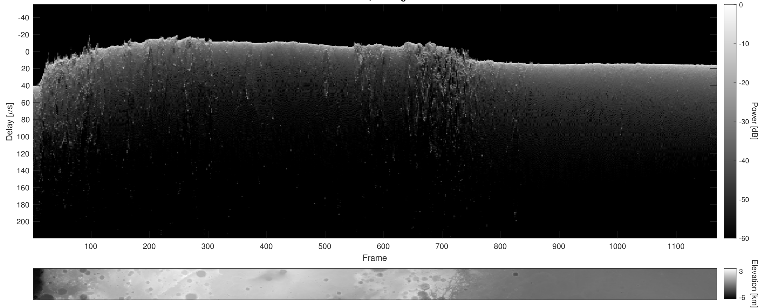
Orbit 6013, Cluttergram
