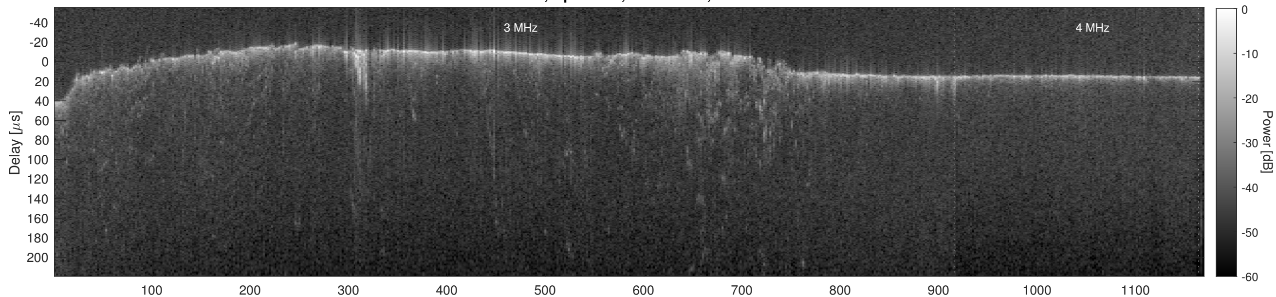
Orbit 6013, Cluttergram
