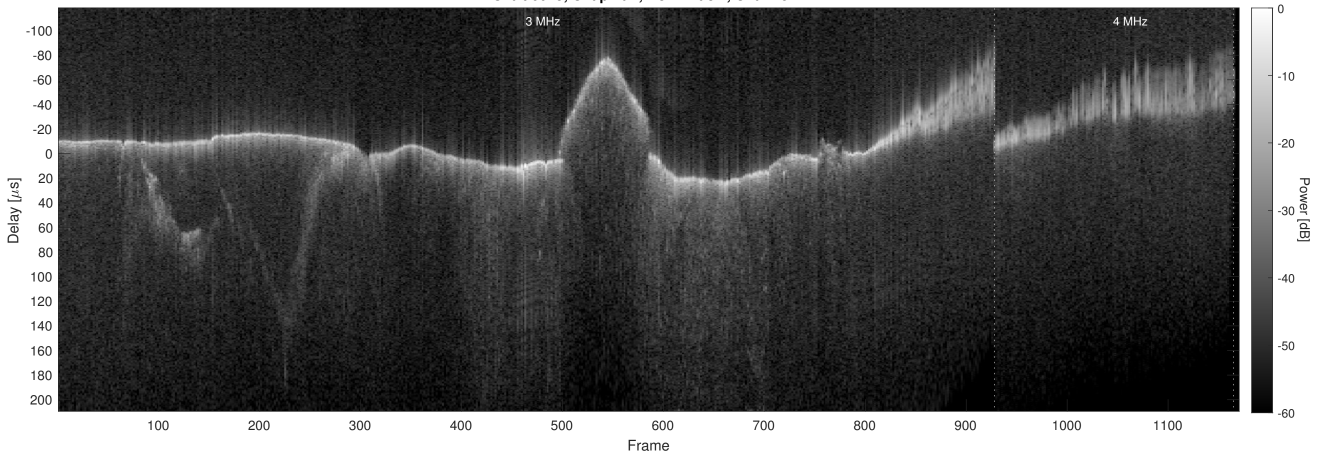
Orbit 6015, Chapman, No Window, Channel 2
