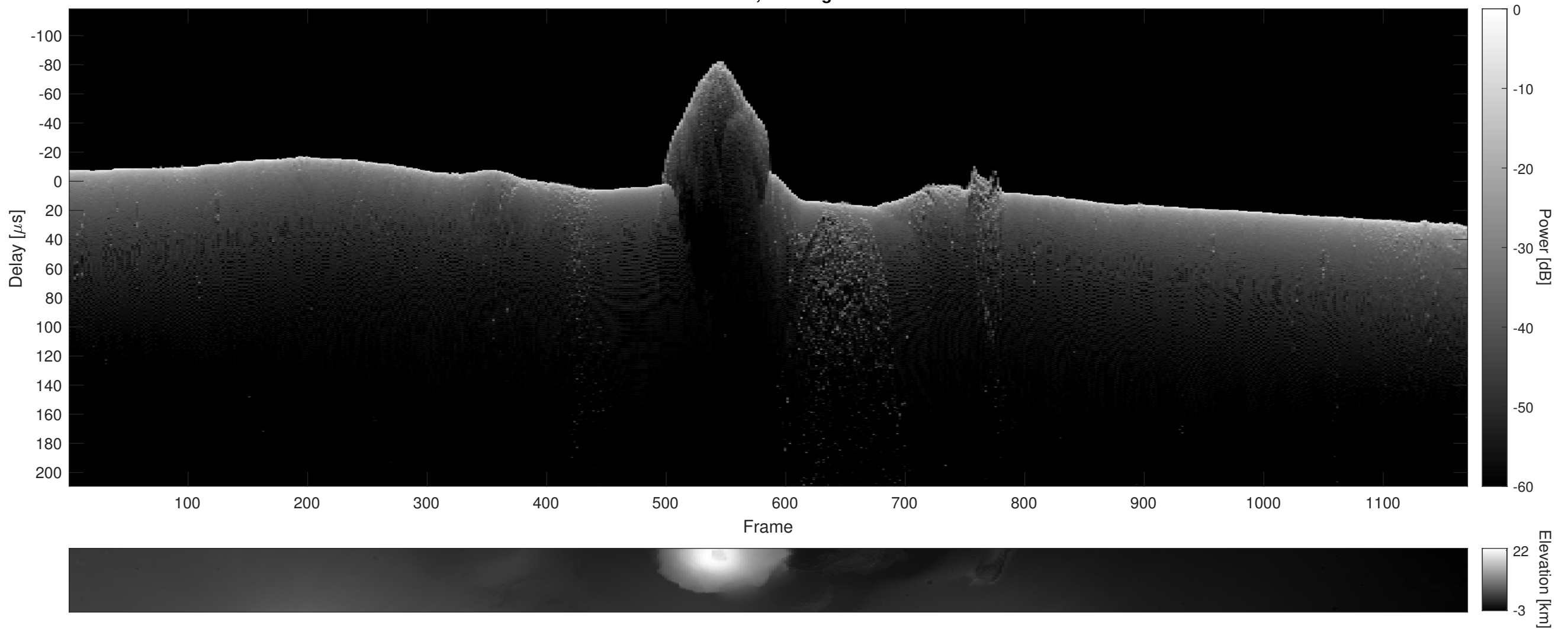
Orbit 6015, Cluttergram
