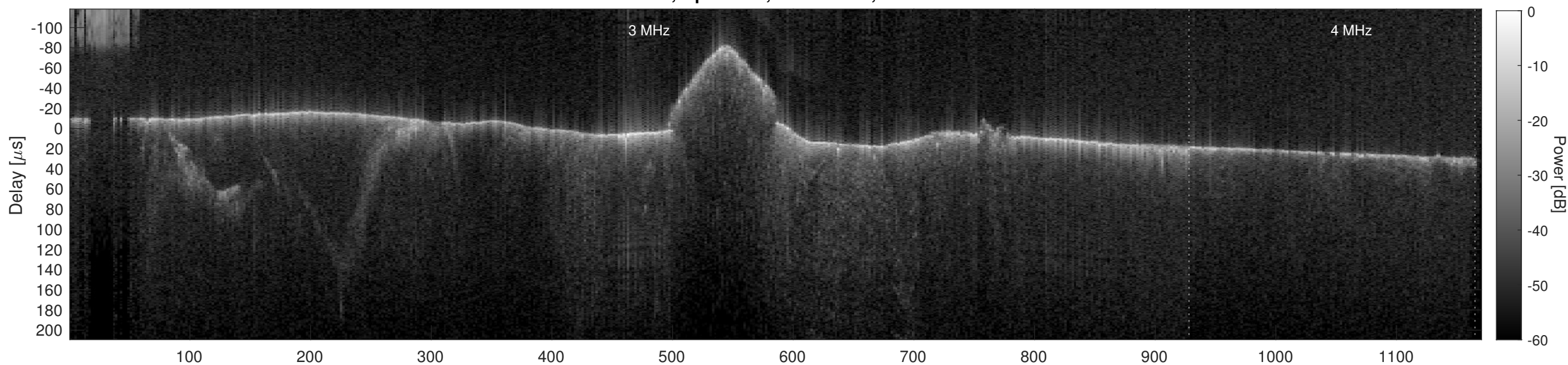
Orbit 6015, Cluttergram
