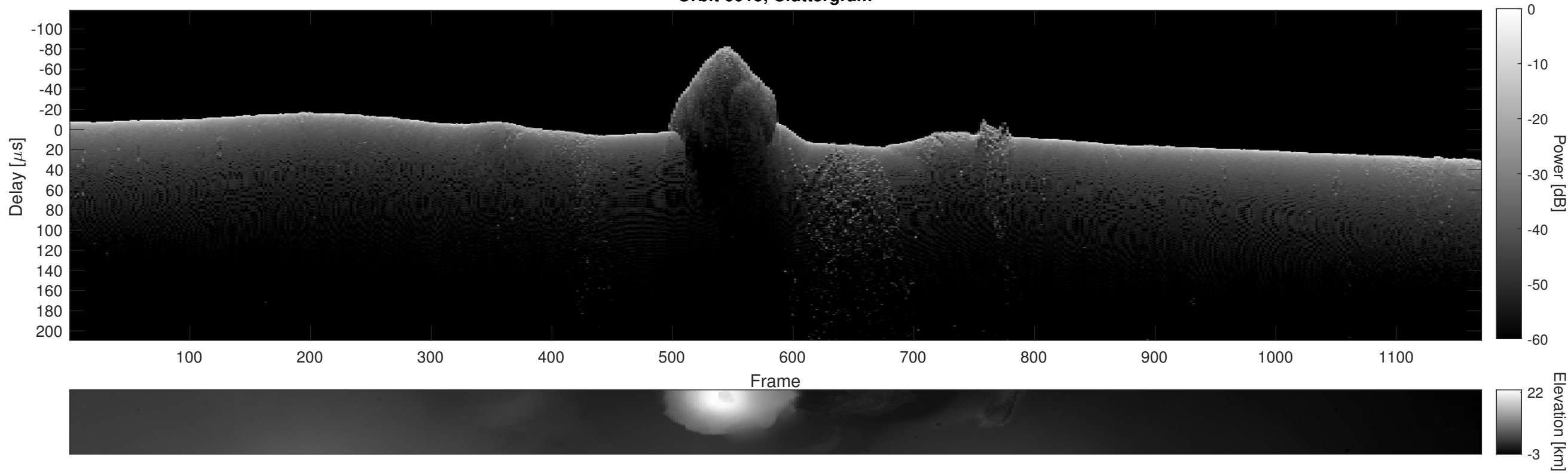
Orbit 6015, Cluttergram
