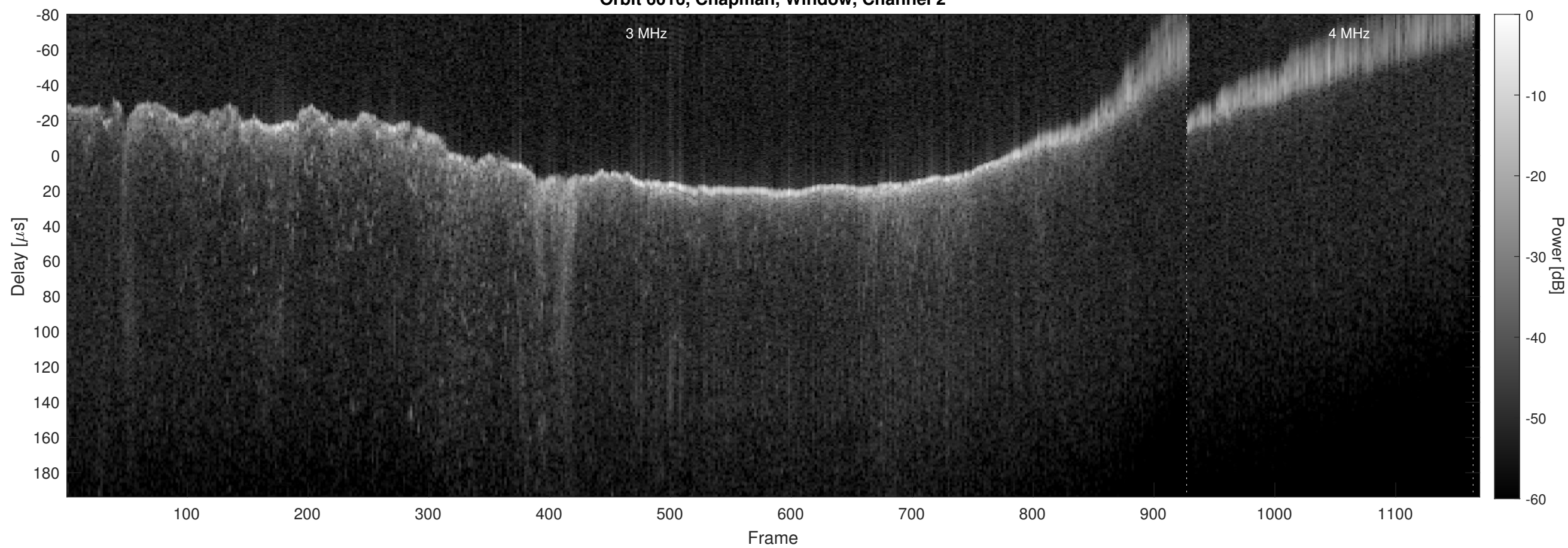
Orbit 6016, Chapman, Window, Channel 2
