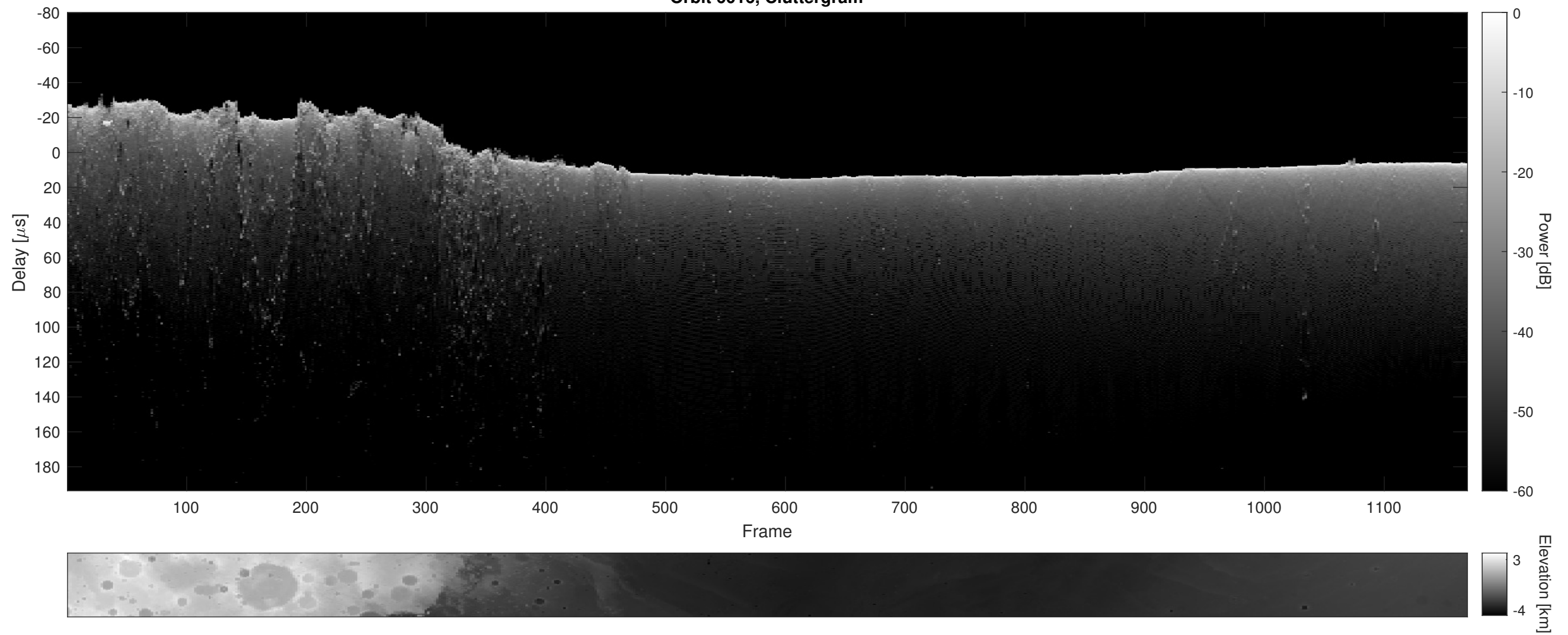
Orbit 6016, Cluttergram
