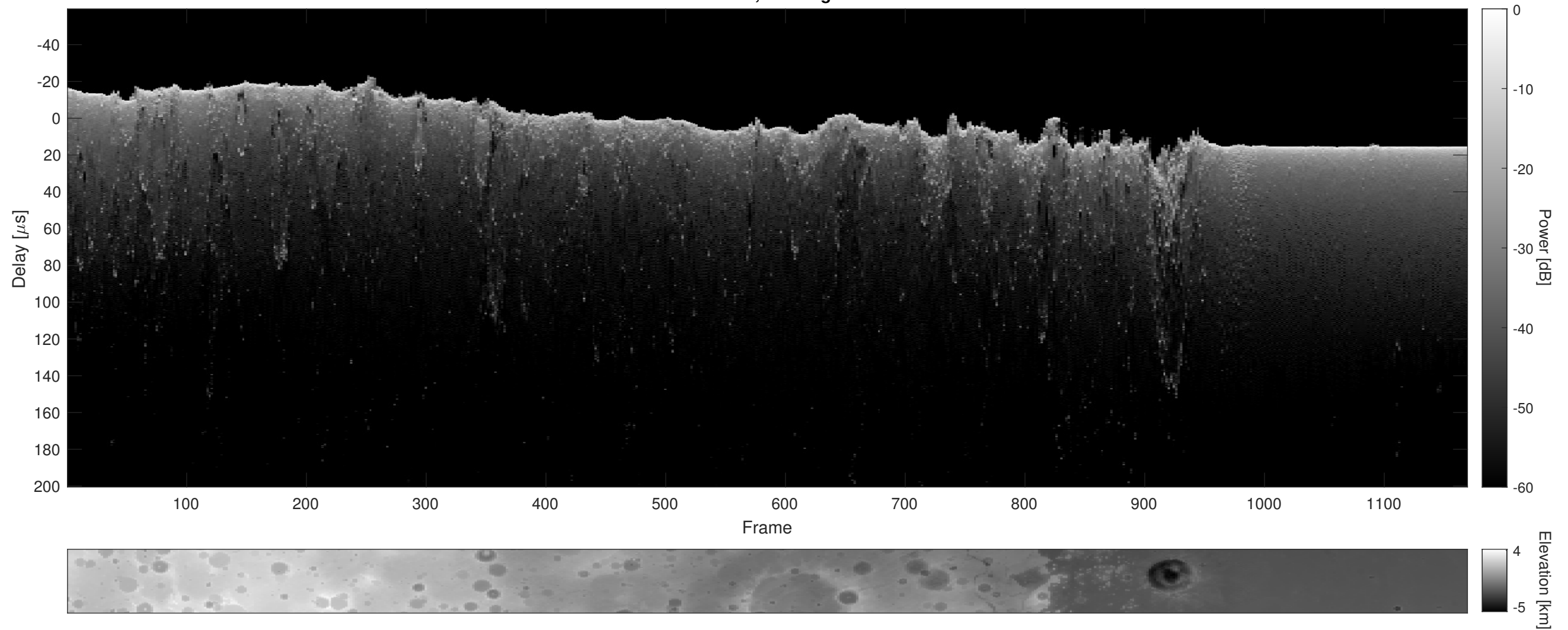
Orbit 6017, Cluttergram
