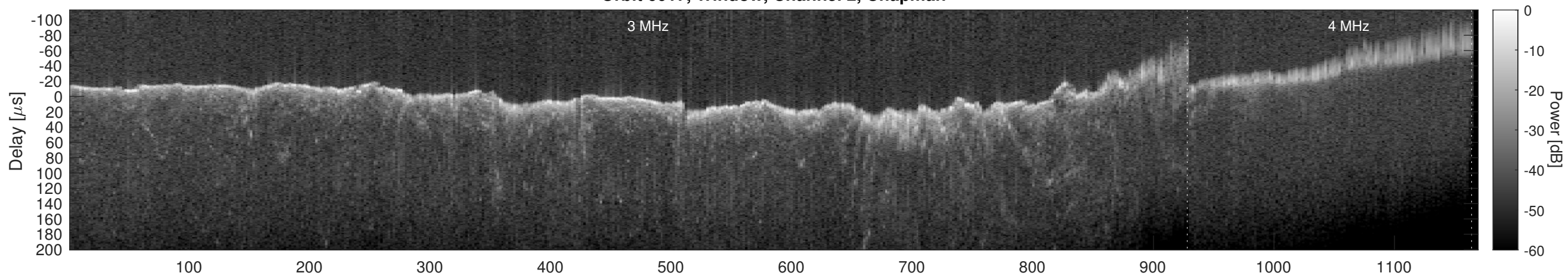
Orbit 6017, Window, Channel 2, Optimized
