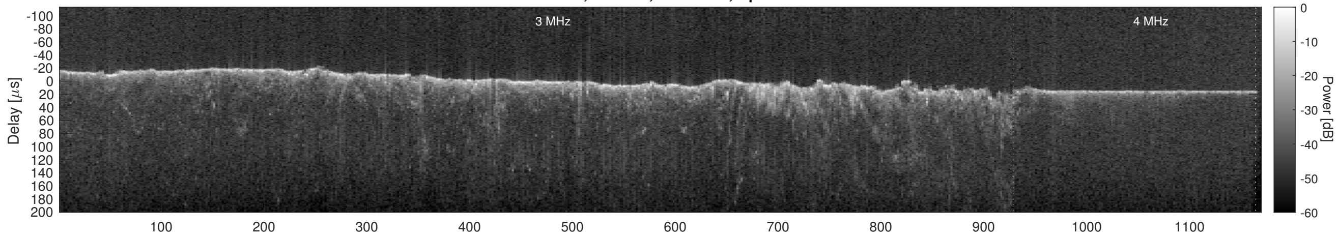
Orbit 6017, Cluttergram
