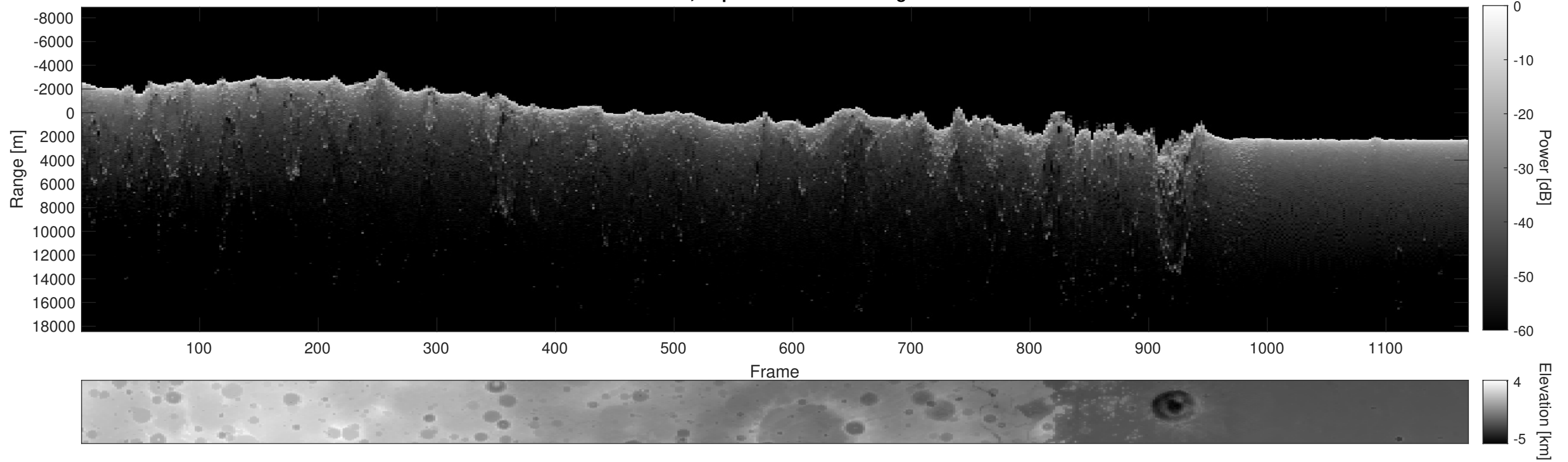
Orbit 6017, Depth-Corrected Cluttergram
