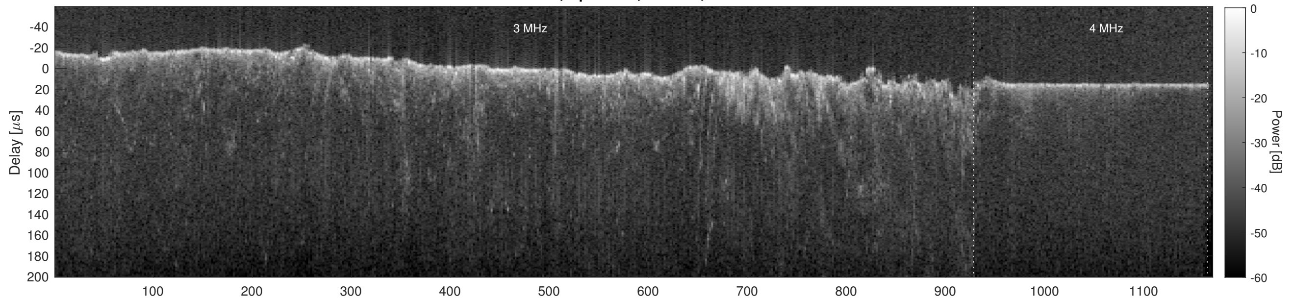
Orbit 6017, Cluttergram
