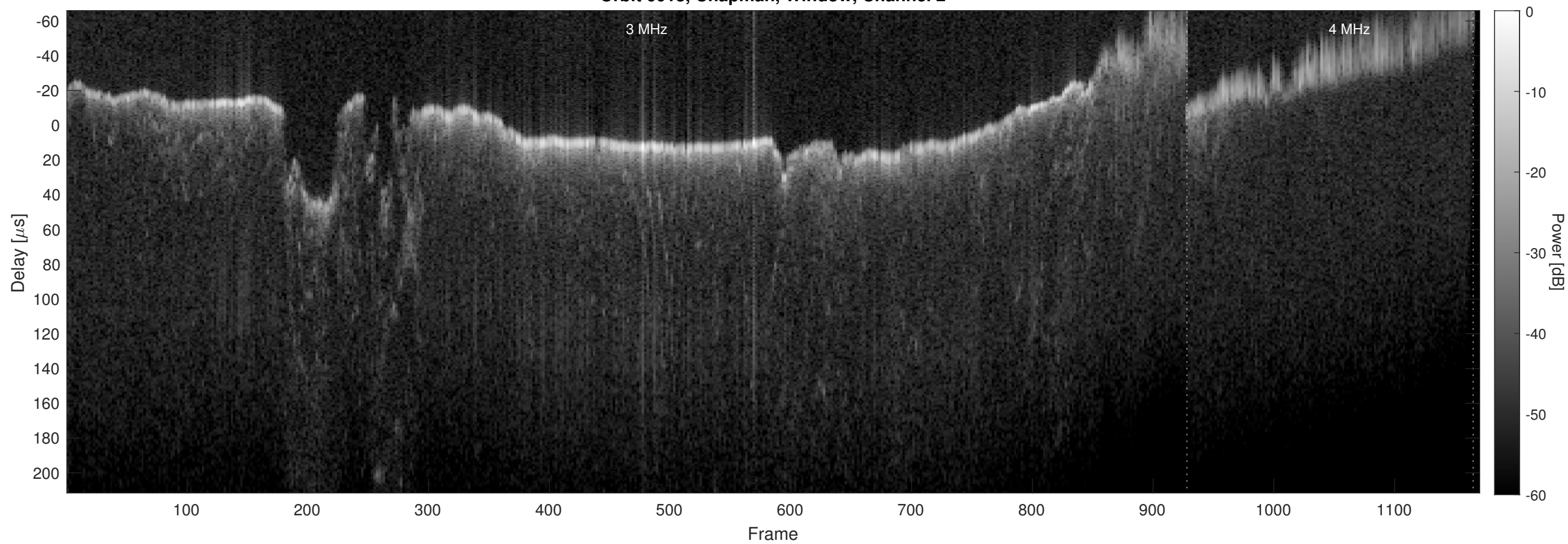
Orbit 6018, Chapman, Window, Channel 2
