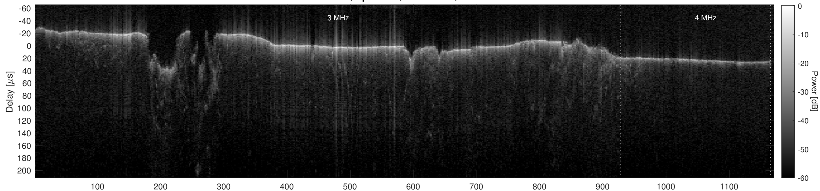
Orbit 6018, Cluttergram
