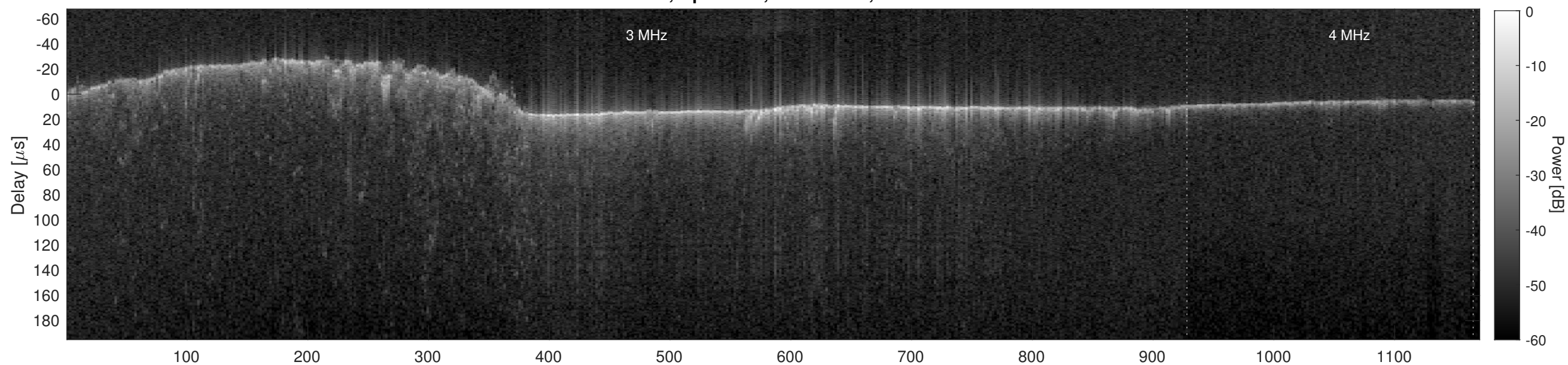
Orbit 6020, Cluttergram
