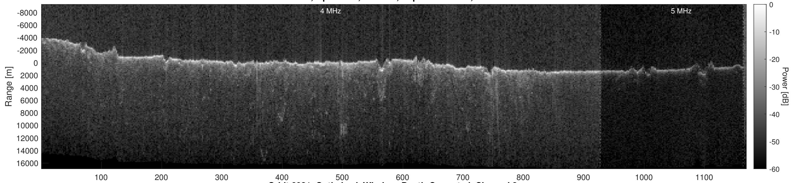
Orbit 6021, Optimized, Window, Depth-Corrected, Channel 2
