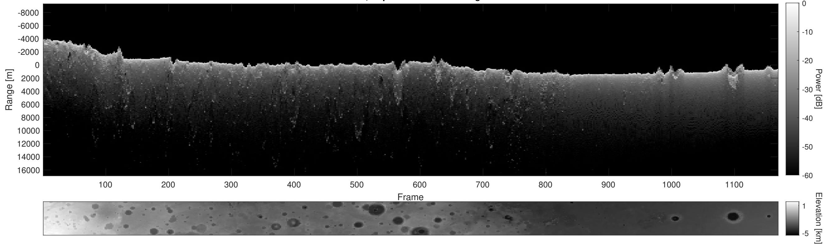
Orbit 6021, Depth-Corrected Cluttergram
