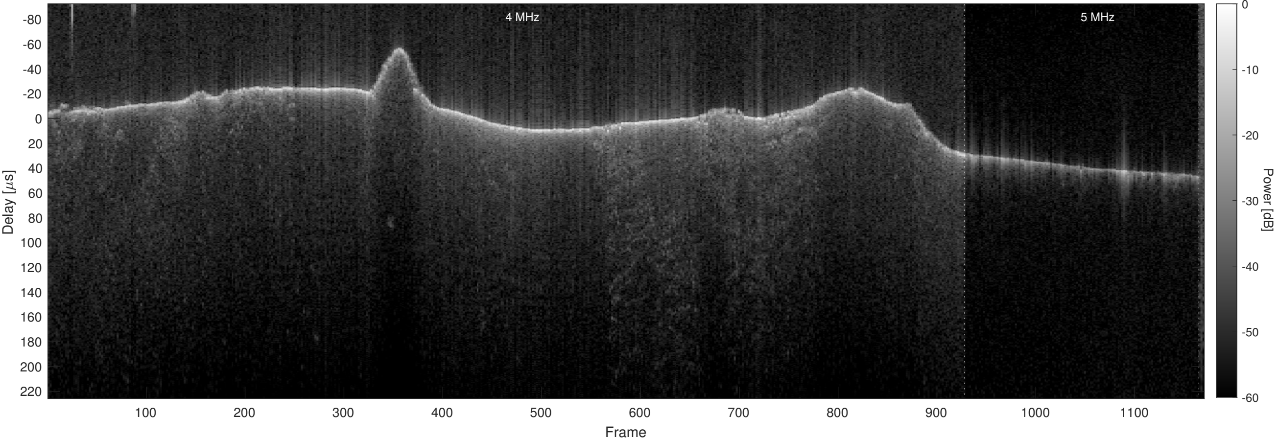
Orbit 6022, Optimized, No Window, Channel 2
