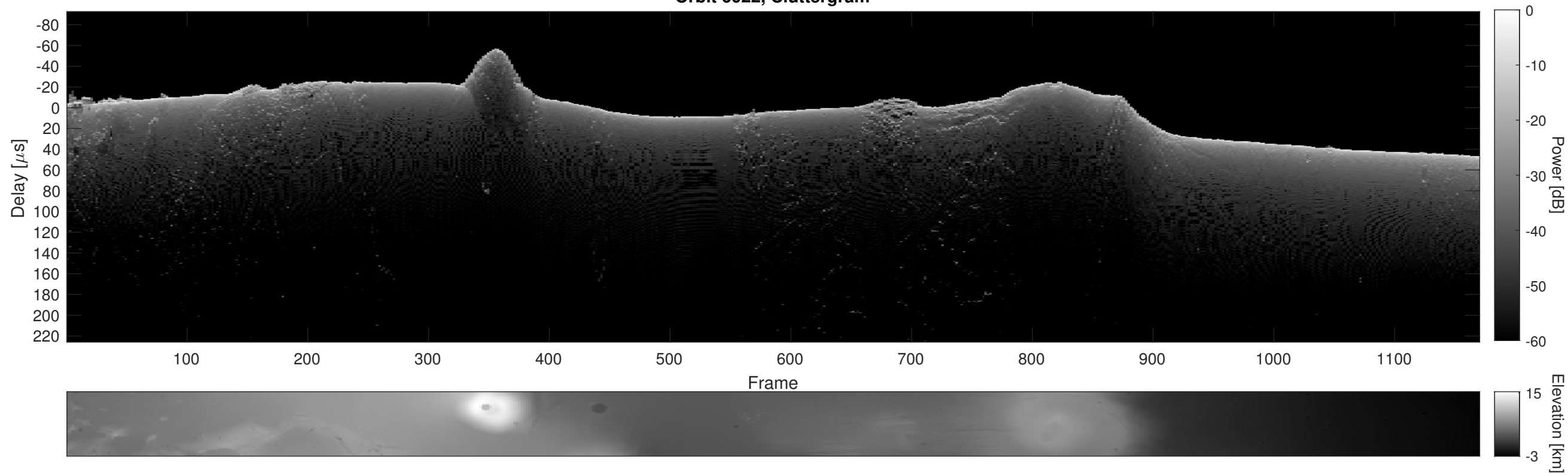
Orbit 6022, Cluttergram
