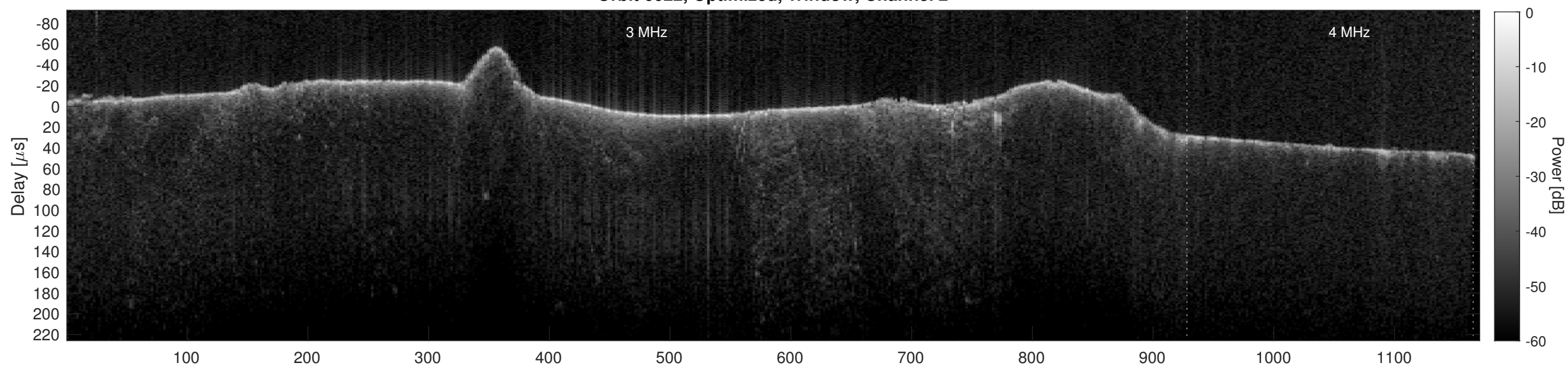
Orbit 6022, Cluttergram
