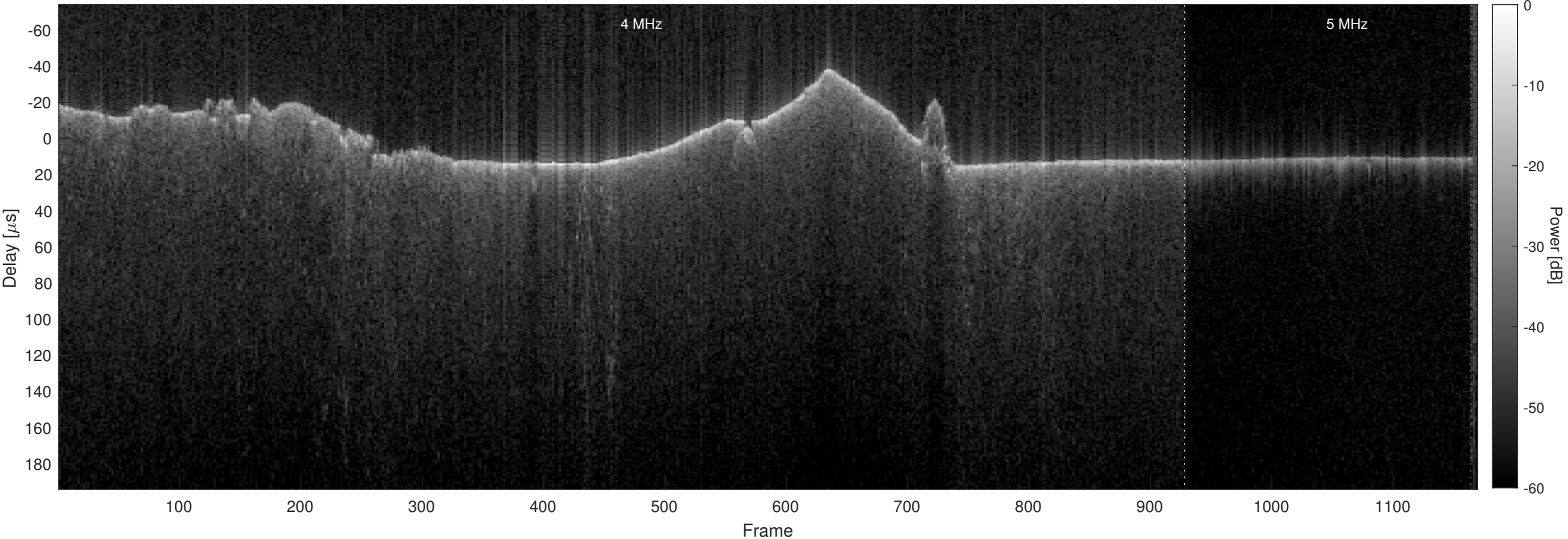
Orbit 6023, Optimized, No Window, Channel 2
