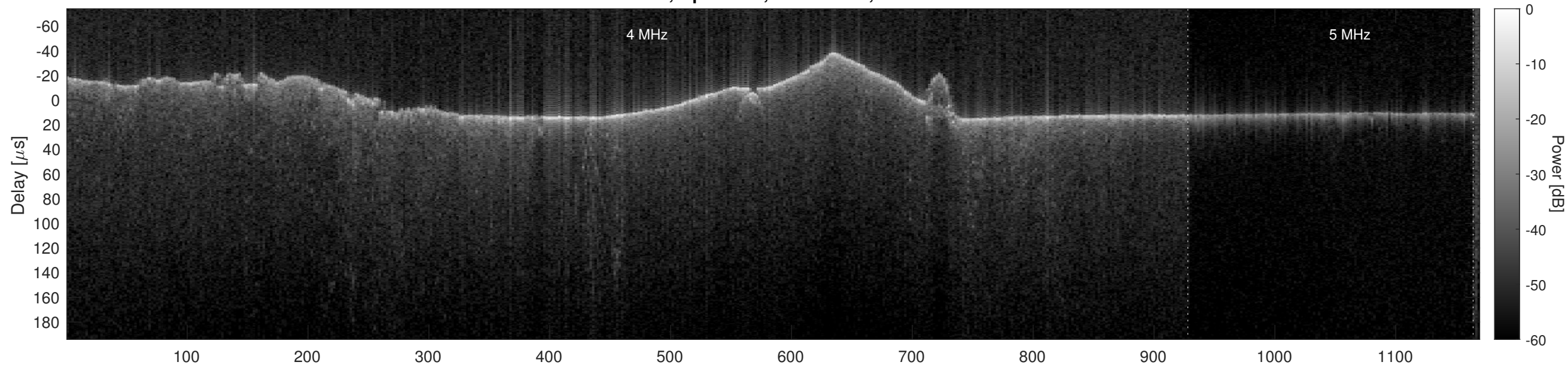
Orbit 6023, Optimized, No Window, Channel 2
