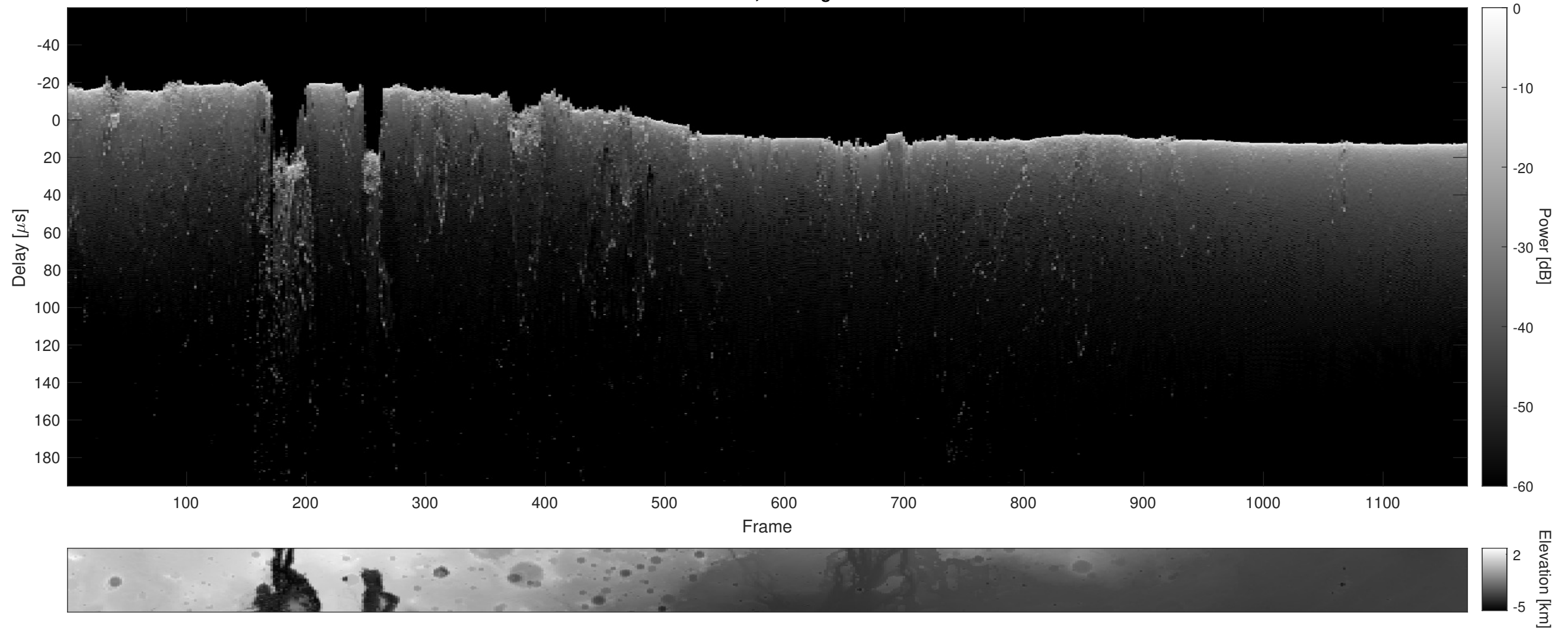
Orbit 6025, Cluttergram
