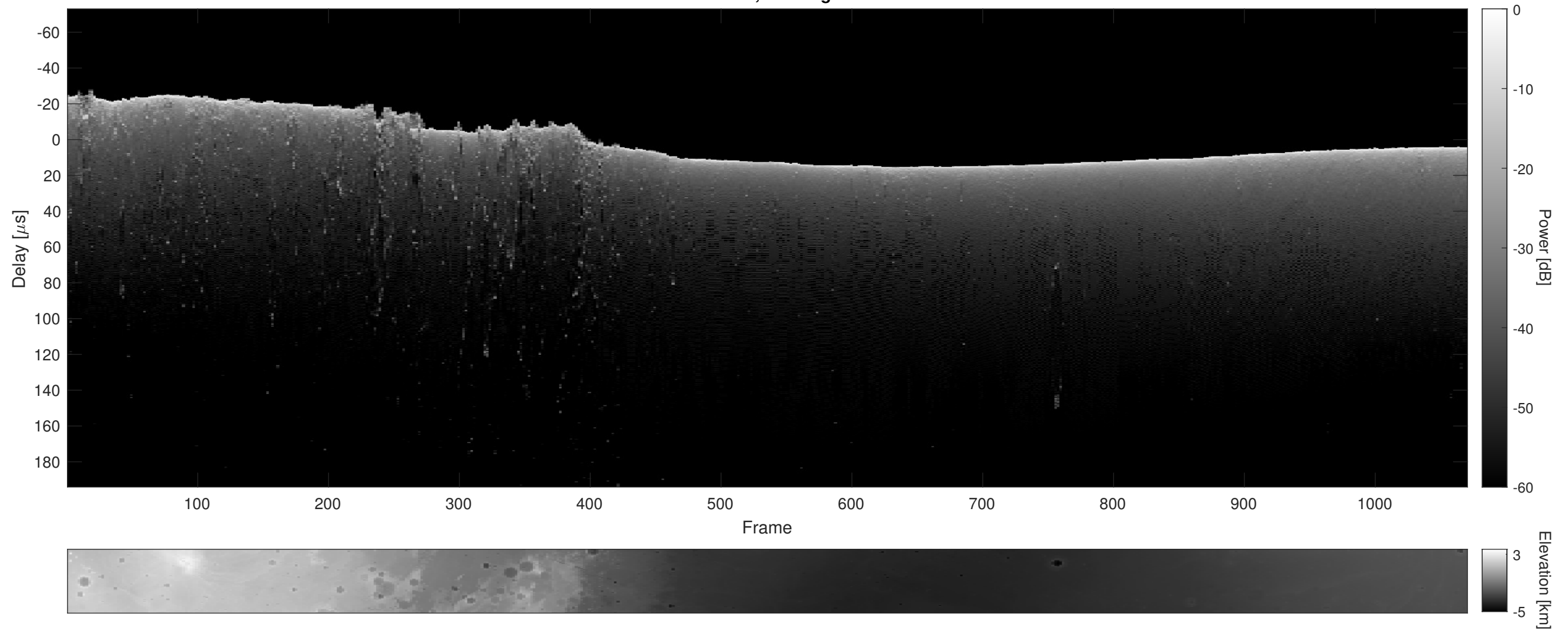
Orbit 6027, Cluttergram
