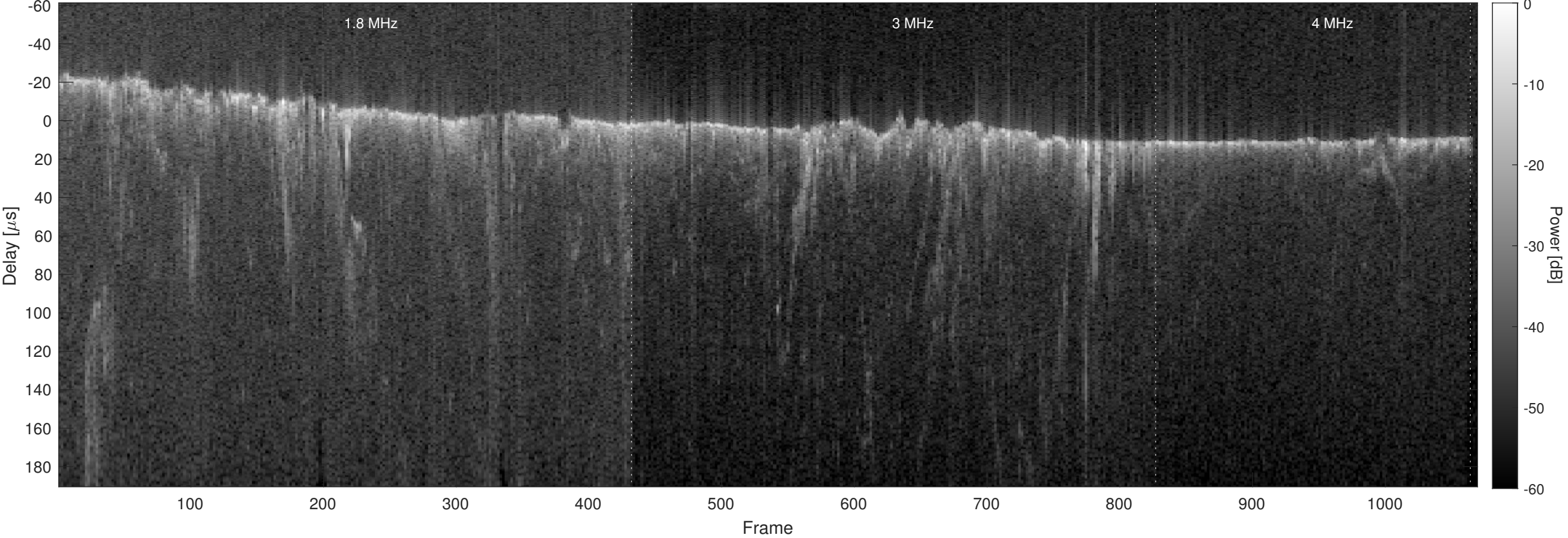
Orbit 6028, Optimized, No Window, Channel 2
