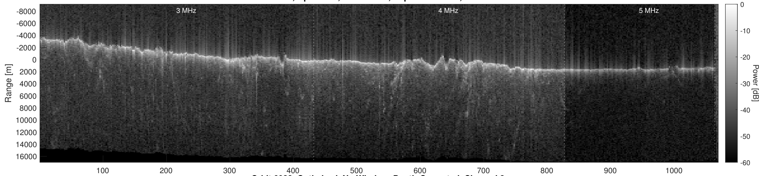
Orbit 6028, Optimized, No Window, Depth-Corrected, Channel 2
