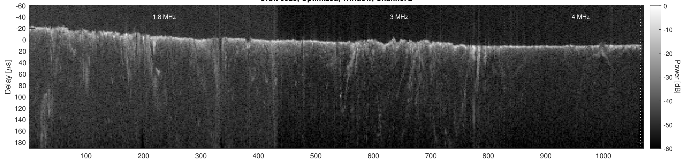
Orbit 6028, Cluttergram
