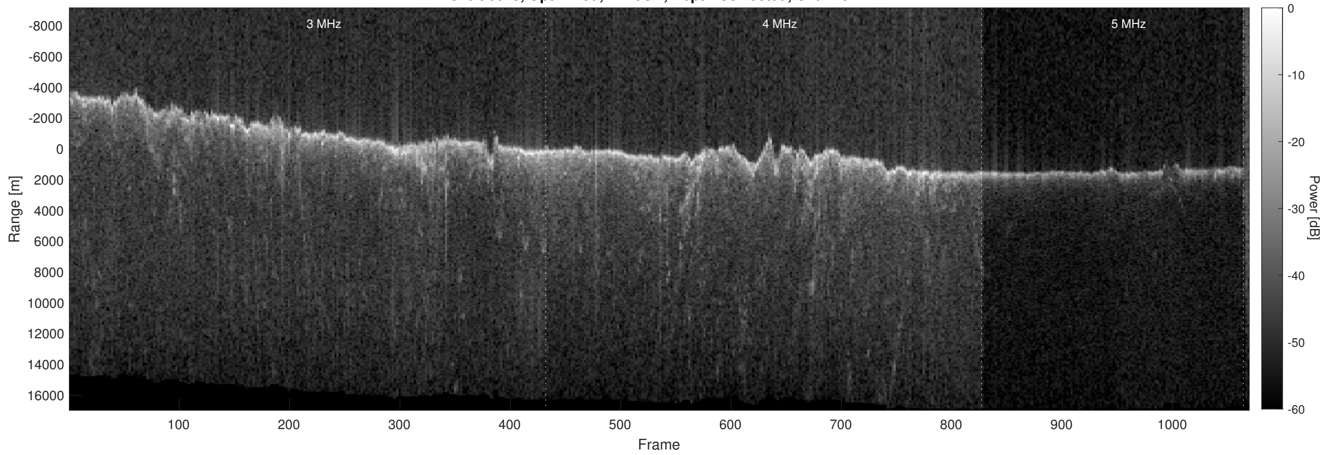
Orbit 6028, Optimized, Window, Depth-Corrected, Channel 2
