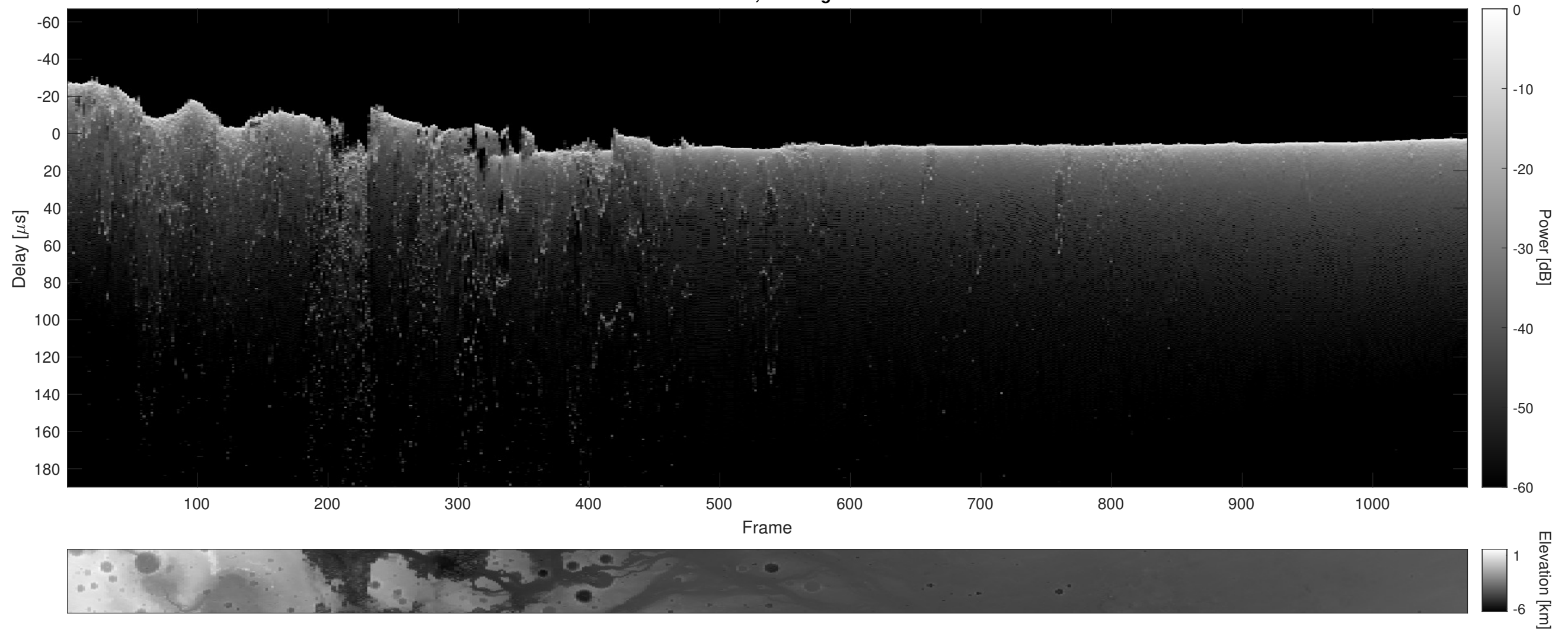
Orbit 6032, Cluttergram
