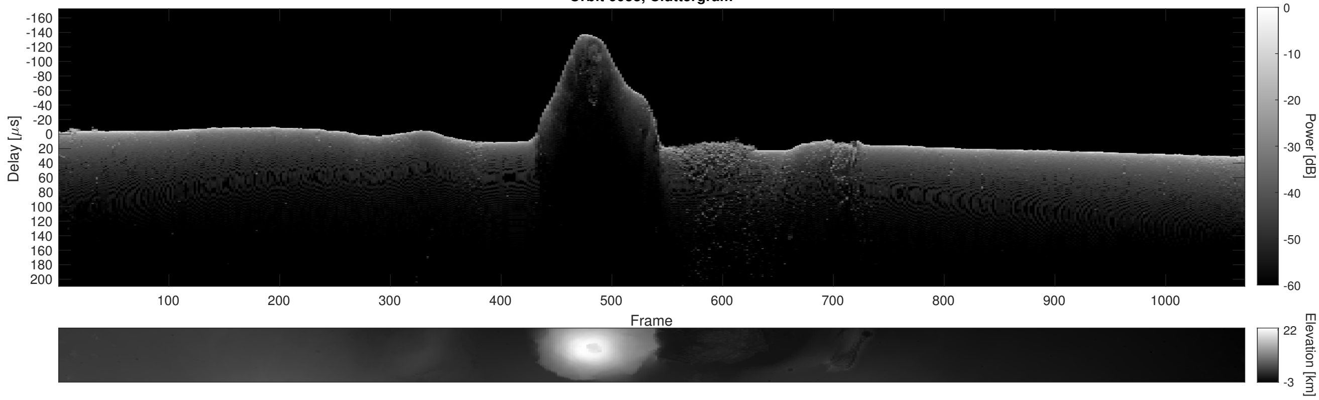
Orbit 6033, Cluttergram
