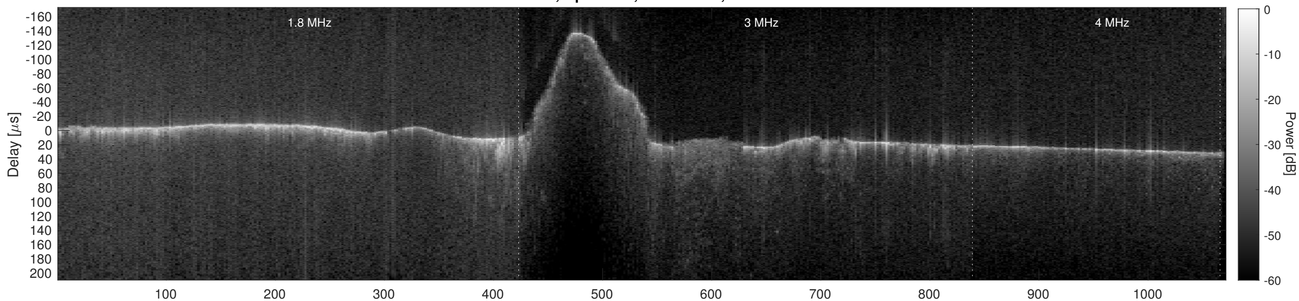
Orbit 6033, Cluttergram
