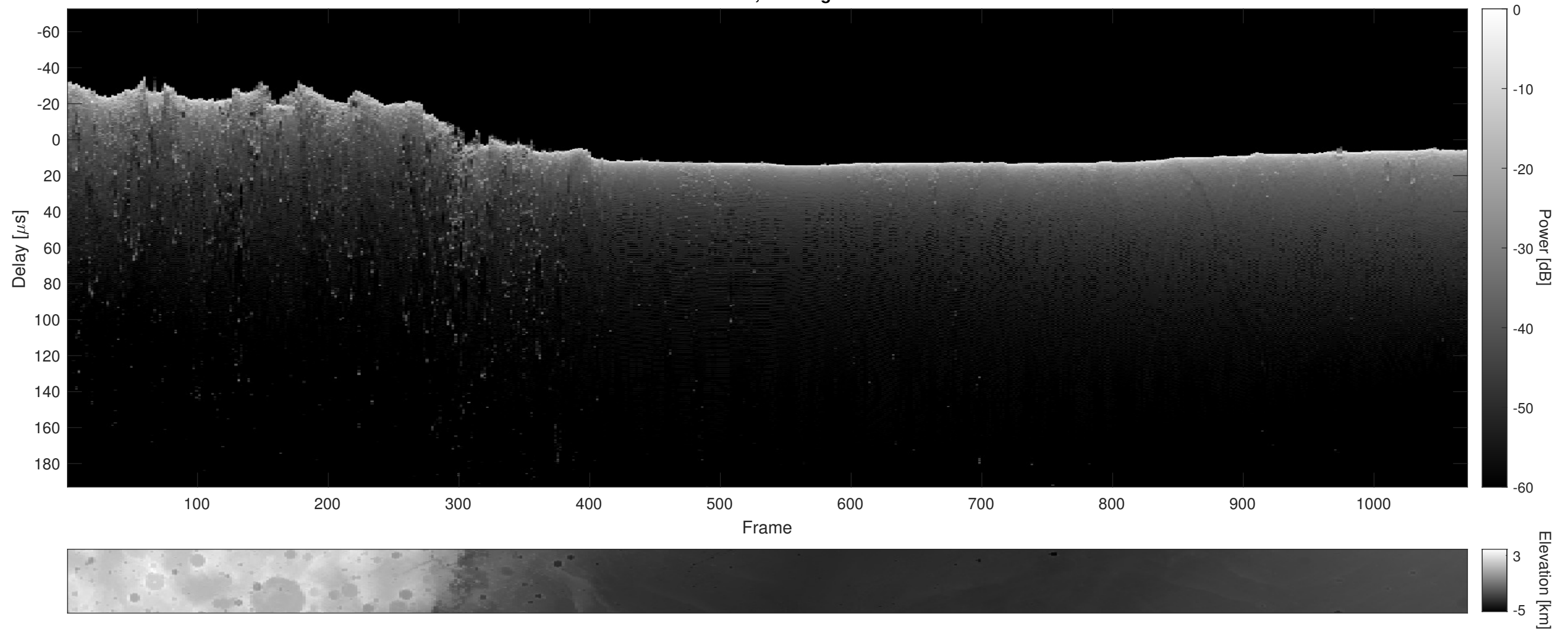
Orbit 6034, Cluttergram
