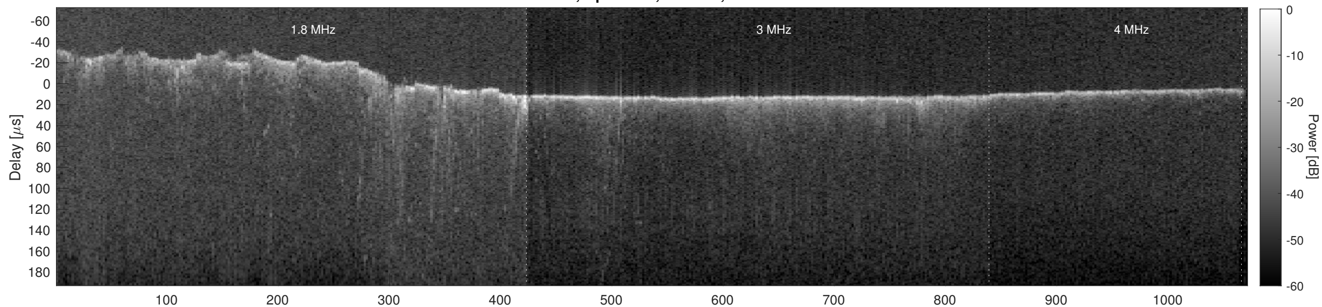
Orbit 6034, Cluttergram
