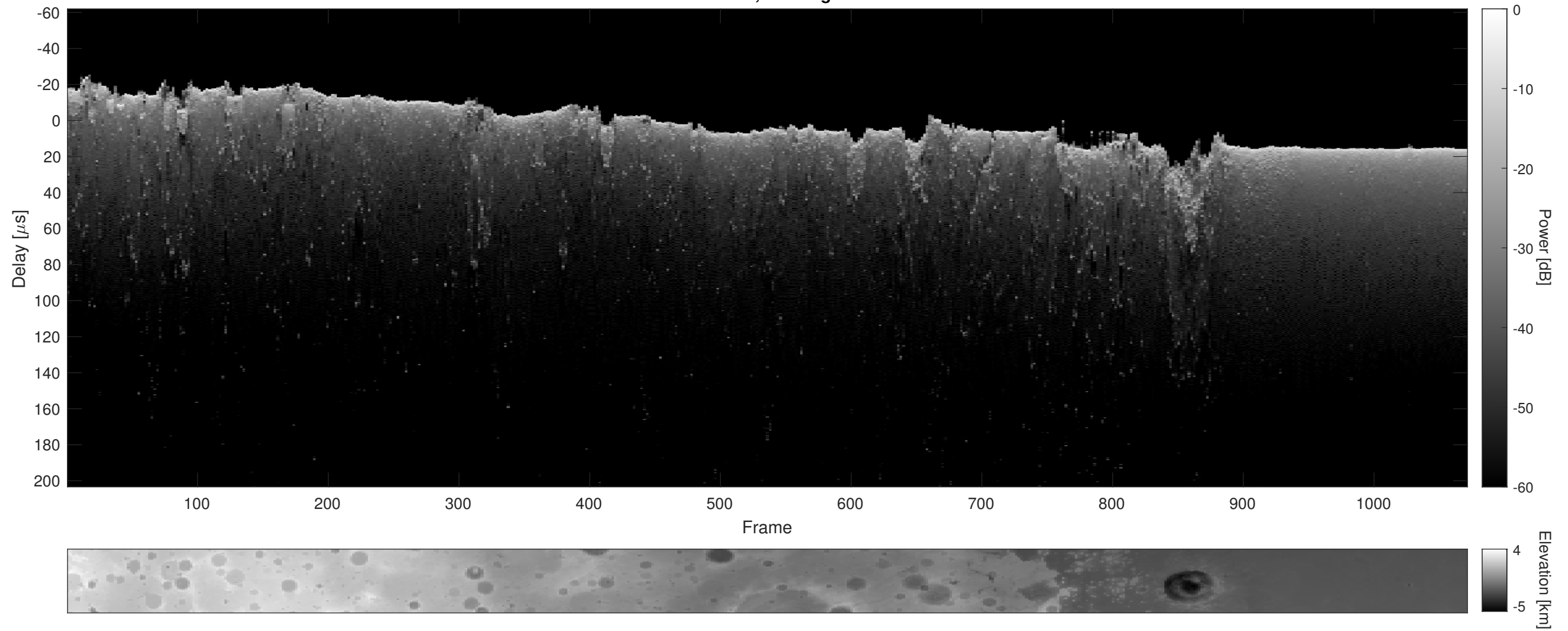
Orbit 6035, Cluttergram
