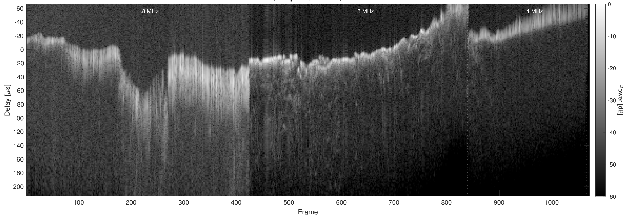
Orbit 6036, Chapman, Window, Channel 2
