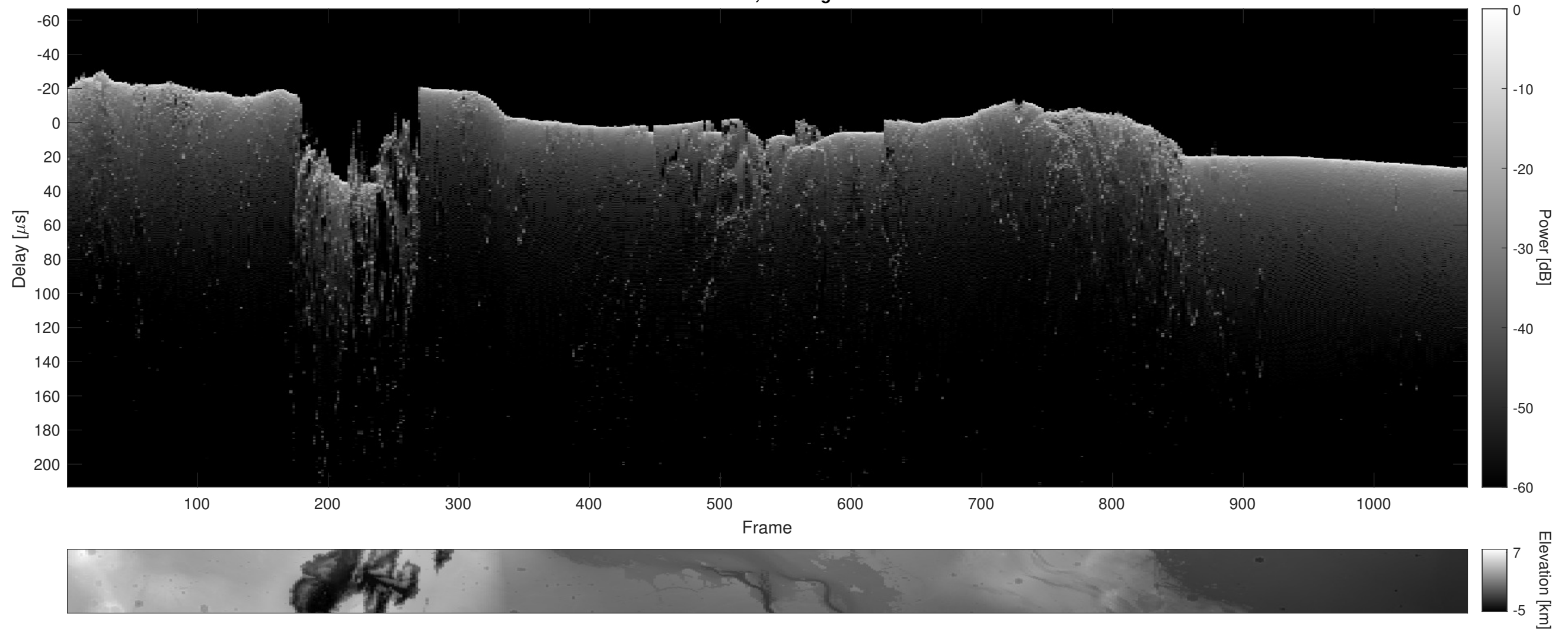
Orbit 6036, Cluttergram
