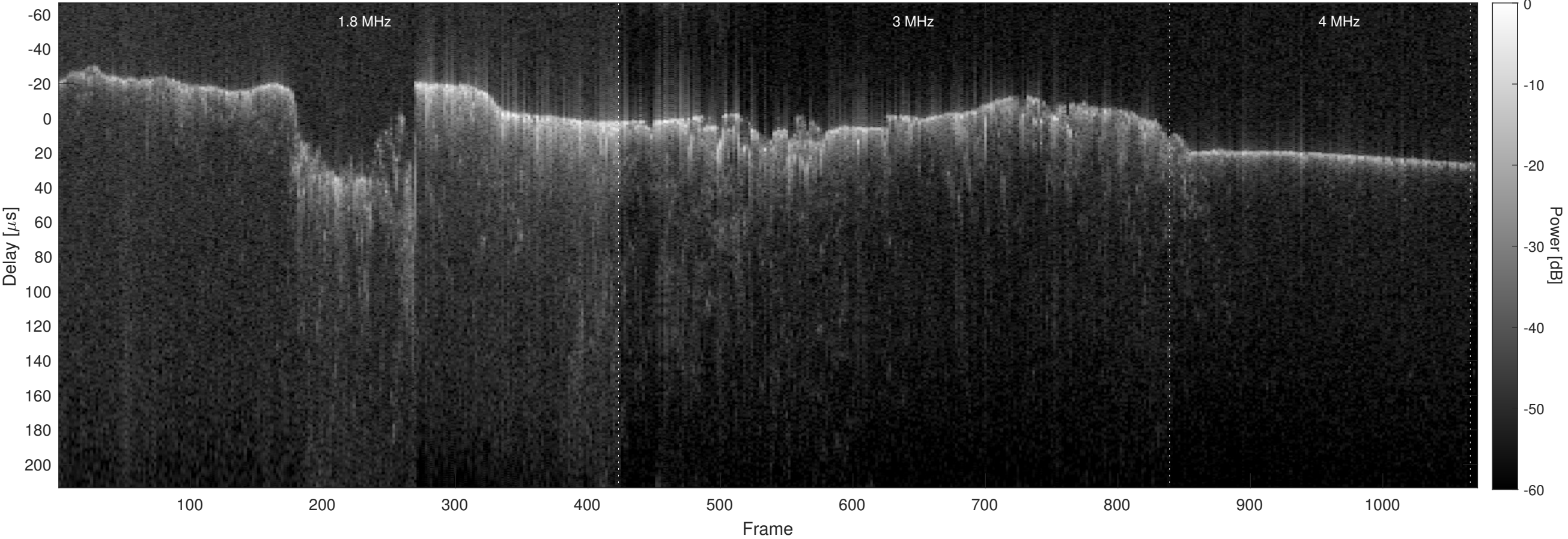
Orbit 6036, Optimized, No Window, Channel 2
