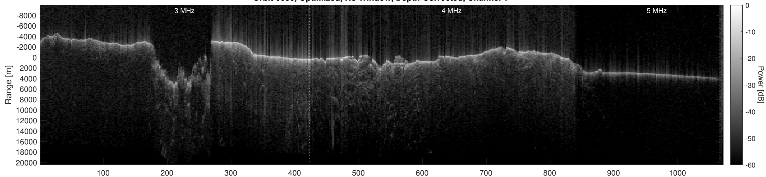
Orbit 6036, Optimized, No Window, Depth-Corrected, Channel 2
