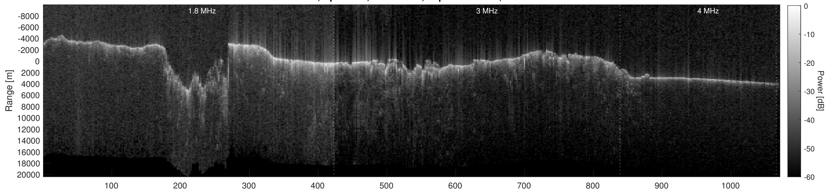
Orbit 6036, Depth-Corrected Cluttergram
