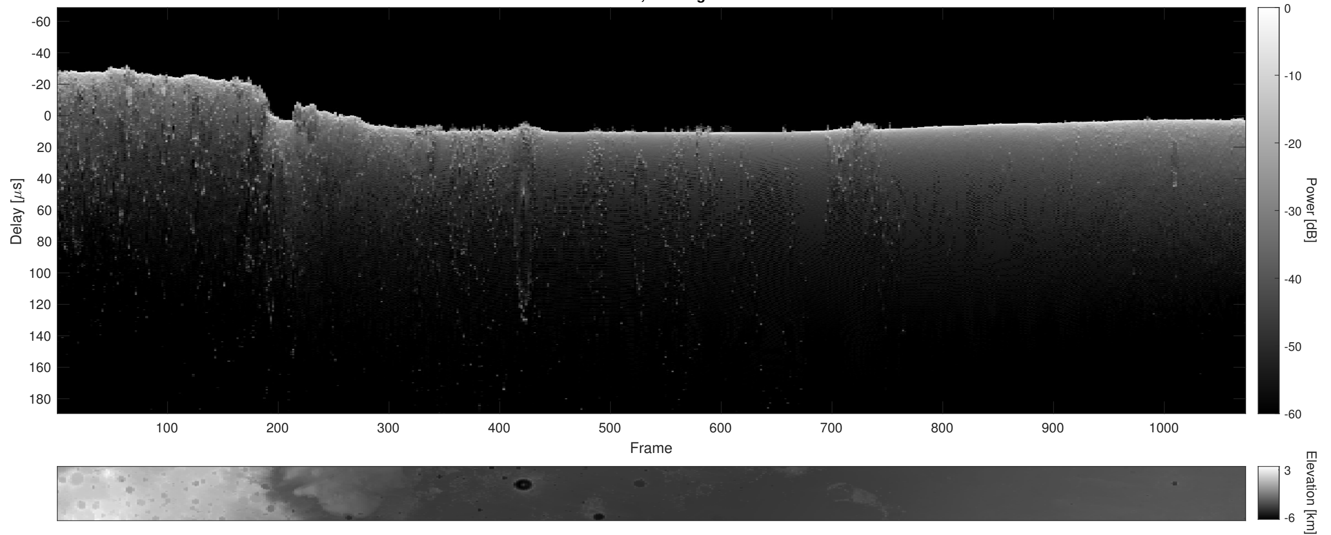
Orbit 6037, Cluttergram
