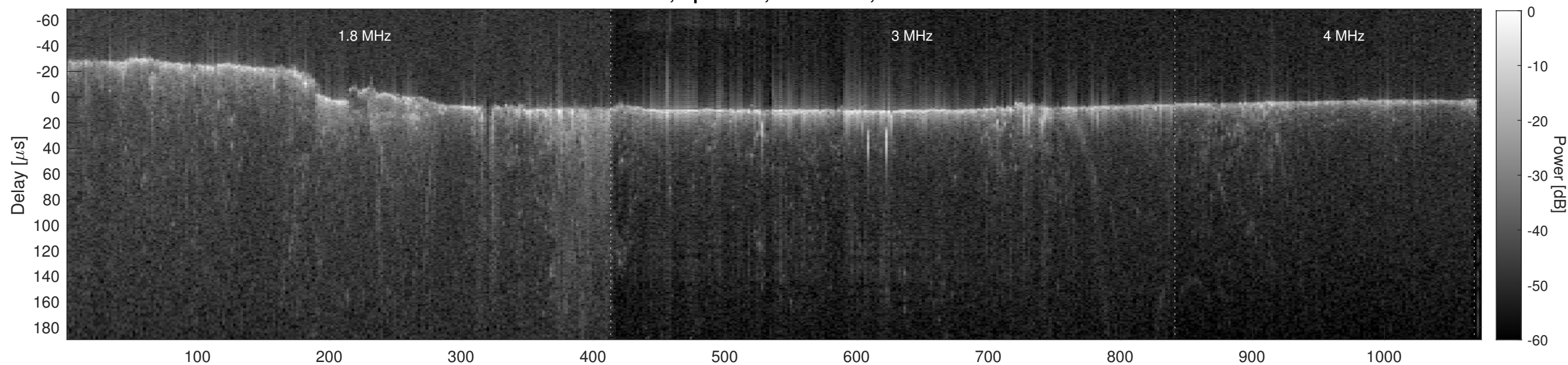
Orbit 6037, Cluttergram
