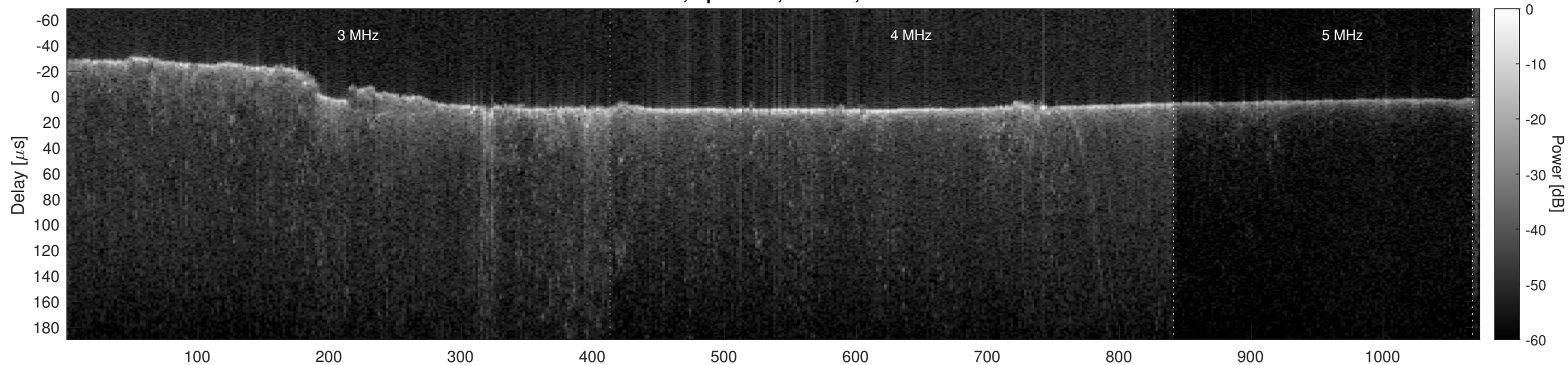
Orbit 6037, Optimized, Window, Channel 2
