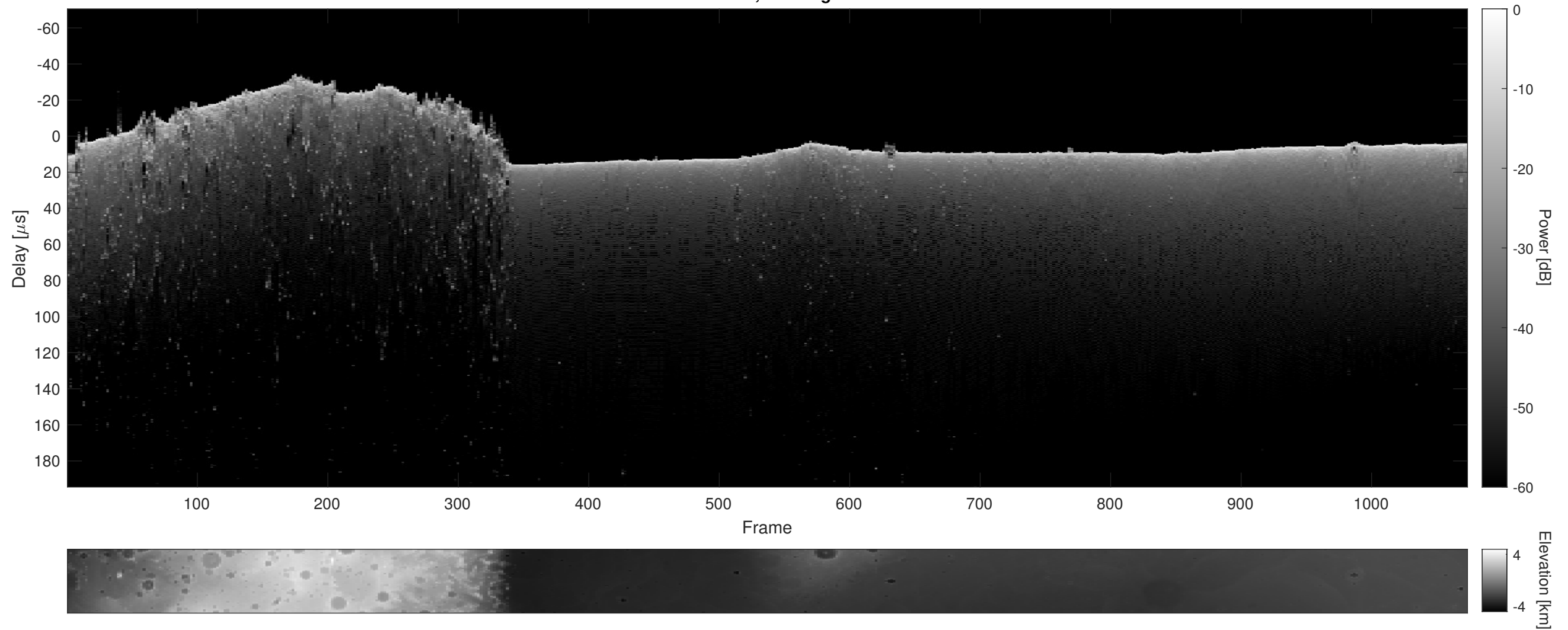
Orbit 6038, Cluttergram
