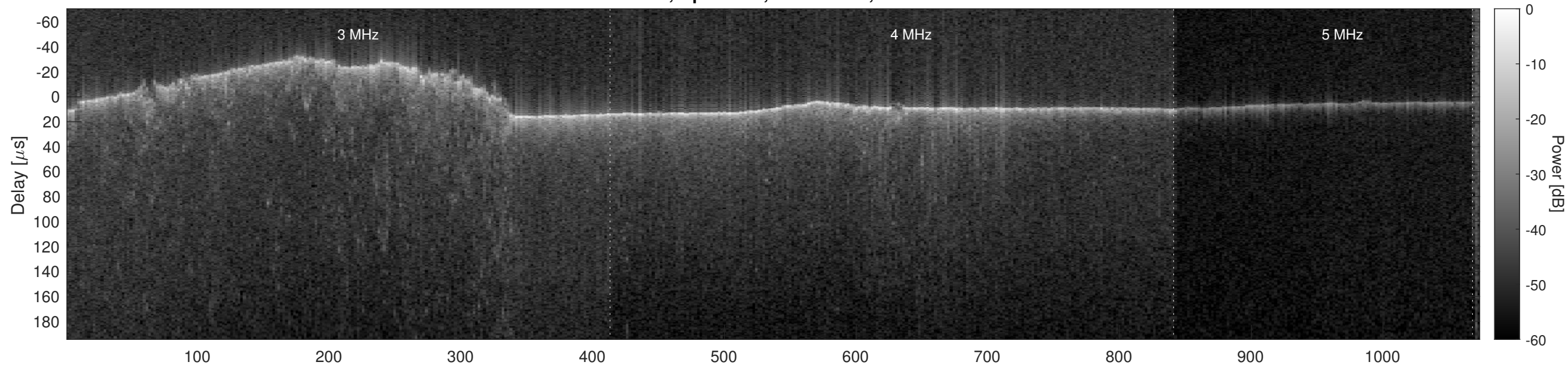
Orbit 6038, Optimized, No Window, Channel 2
