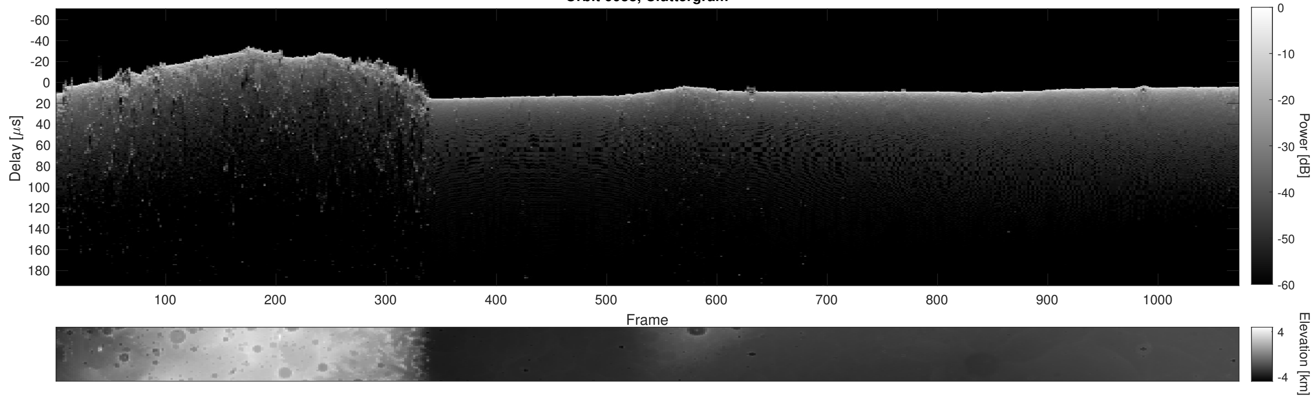
Orbit 6038, Cluttergram
