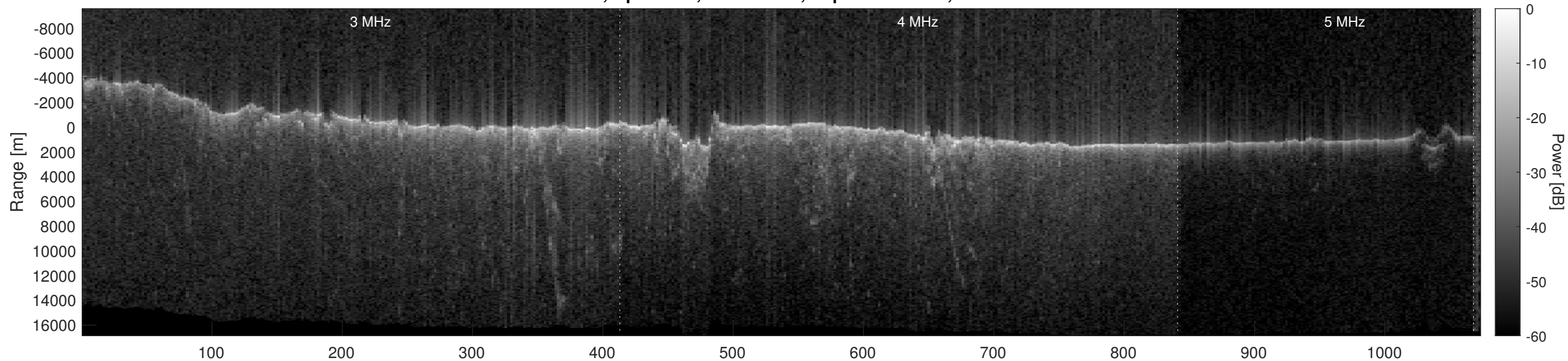
Orbit 6039, Optimized, No Window, Depth-Corrected, Channel 2
