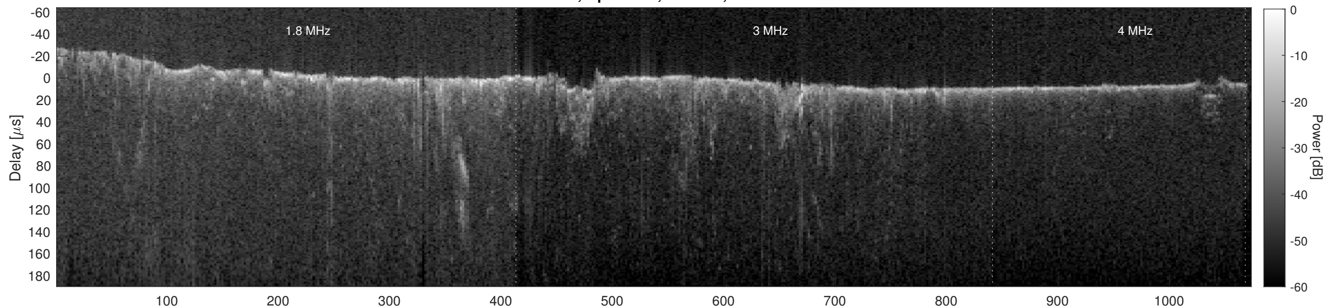
Orbit 6039, Cluttergram
