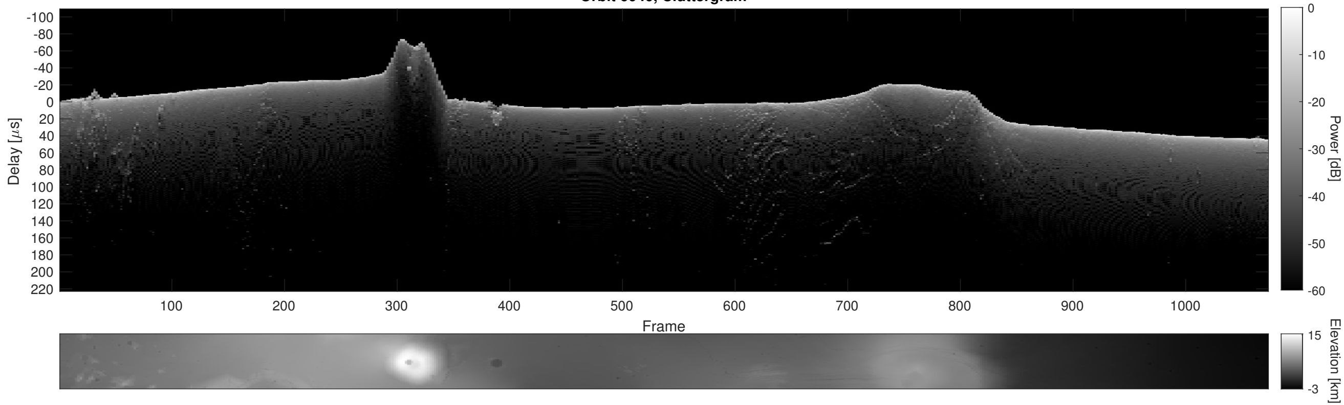
Orbit 6040, Cluttergram
