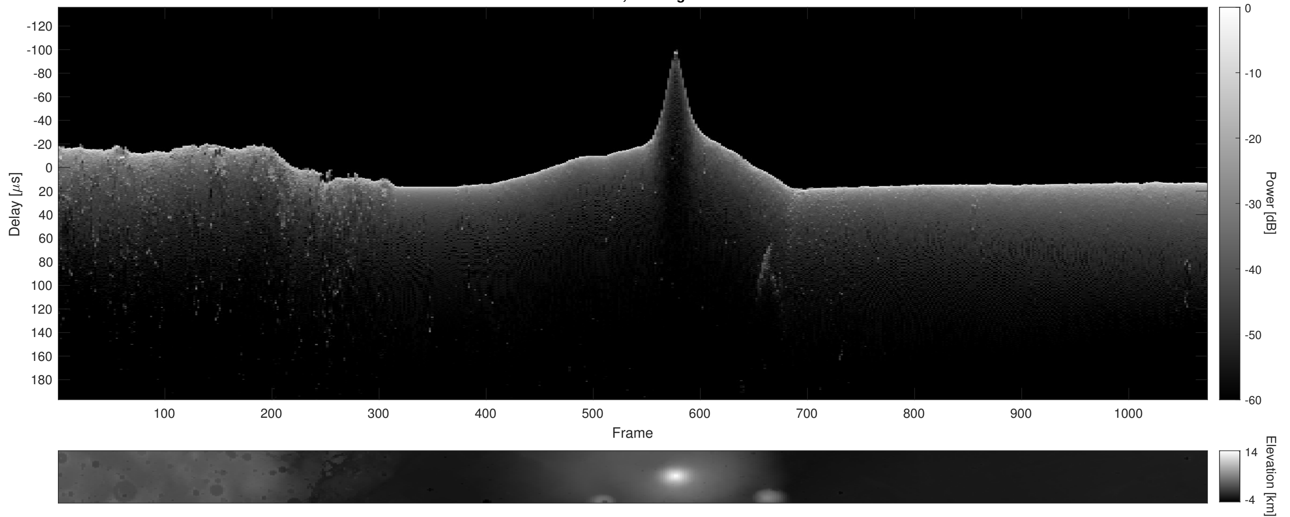
Orbit 6041, Cluttergram
