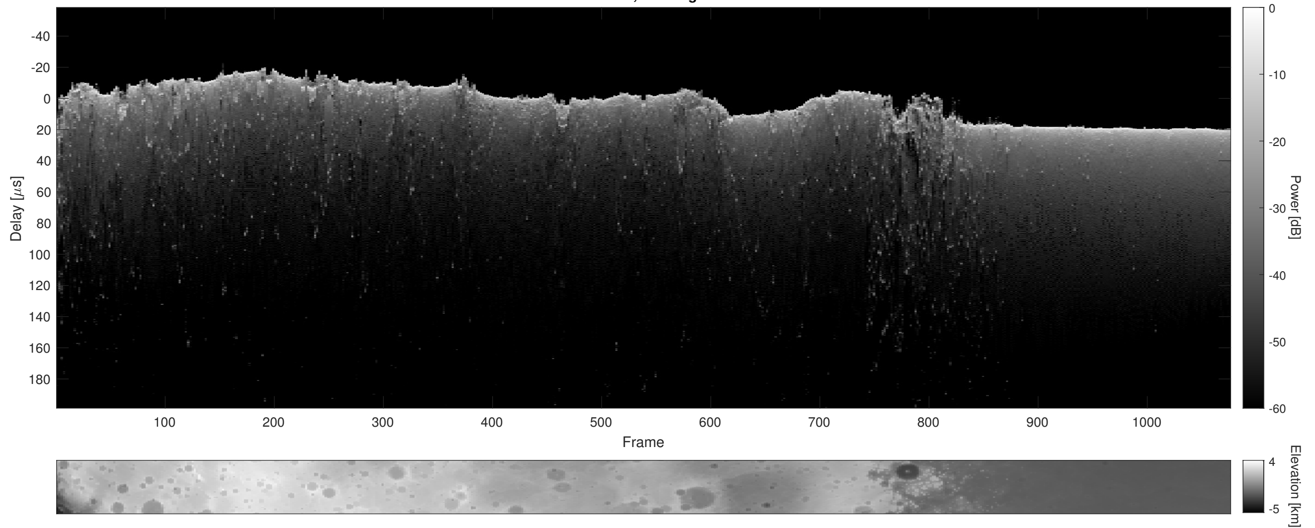
Orbit 6042, Cluttergram
