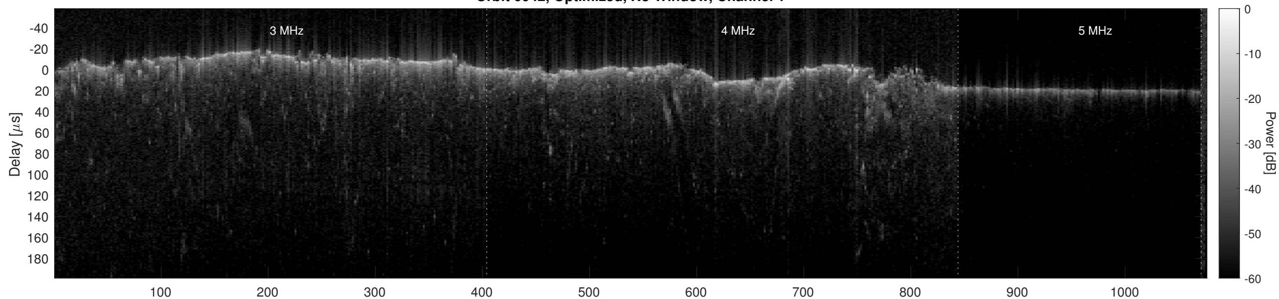
Orbit 6042, Optimized, No Window, Channel 2
