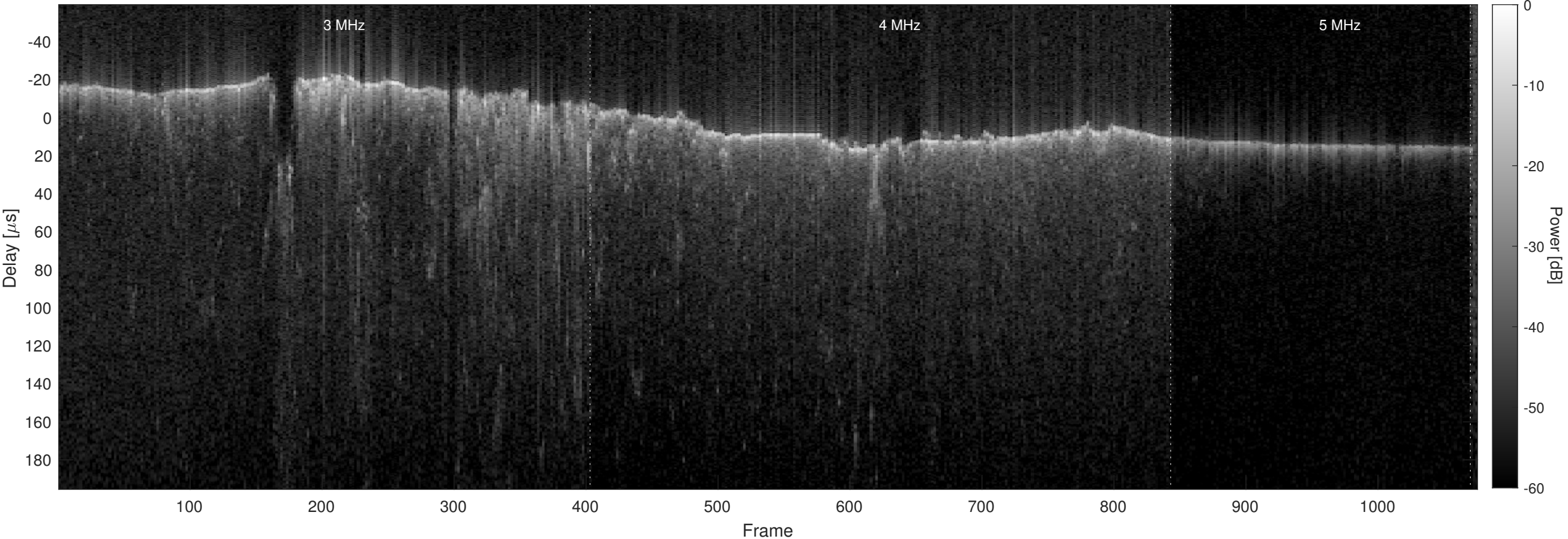
Orbit 6043, Optimized, No Window, Channel 2
