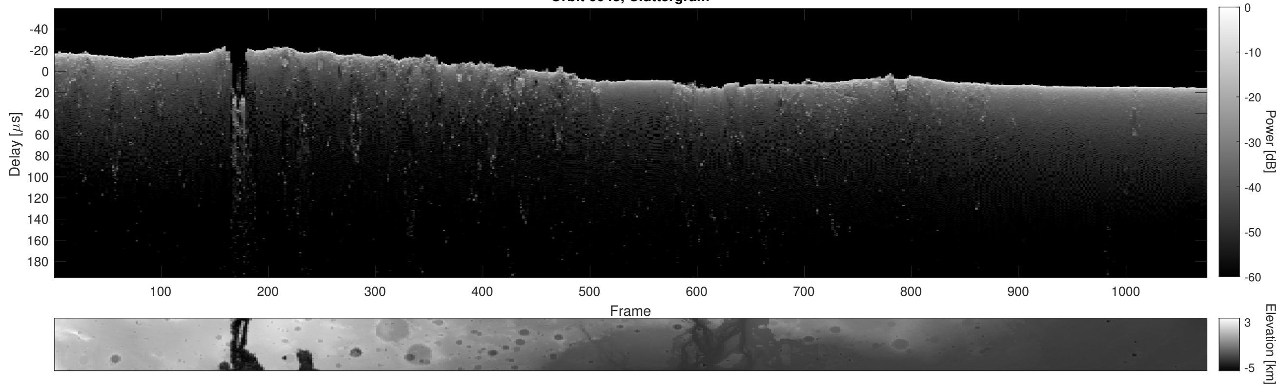
Orbit 6043, Cluttergram
